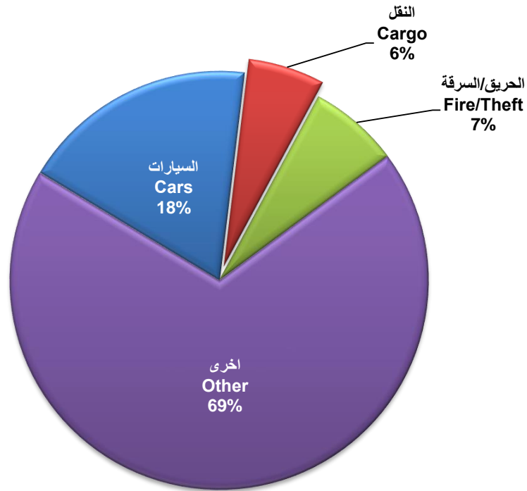
شكل (29) Graph
